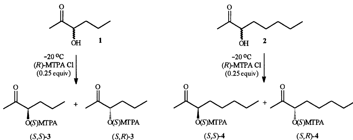
Scheme 1. Kinetically controlled acylations of racemic 3-hydroxy-2-hexanone ( 1 ) and 3-hydroxy-2-octanone ( 2 ).
