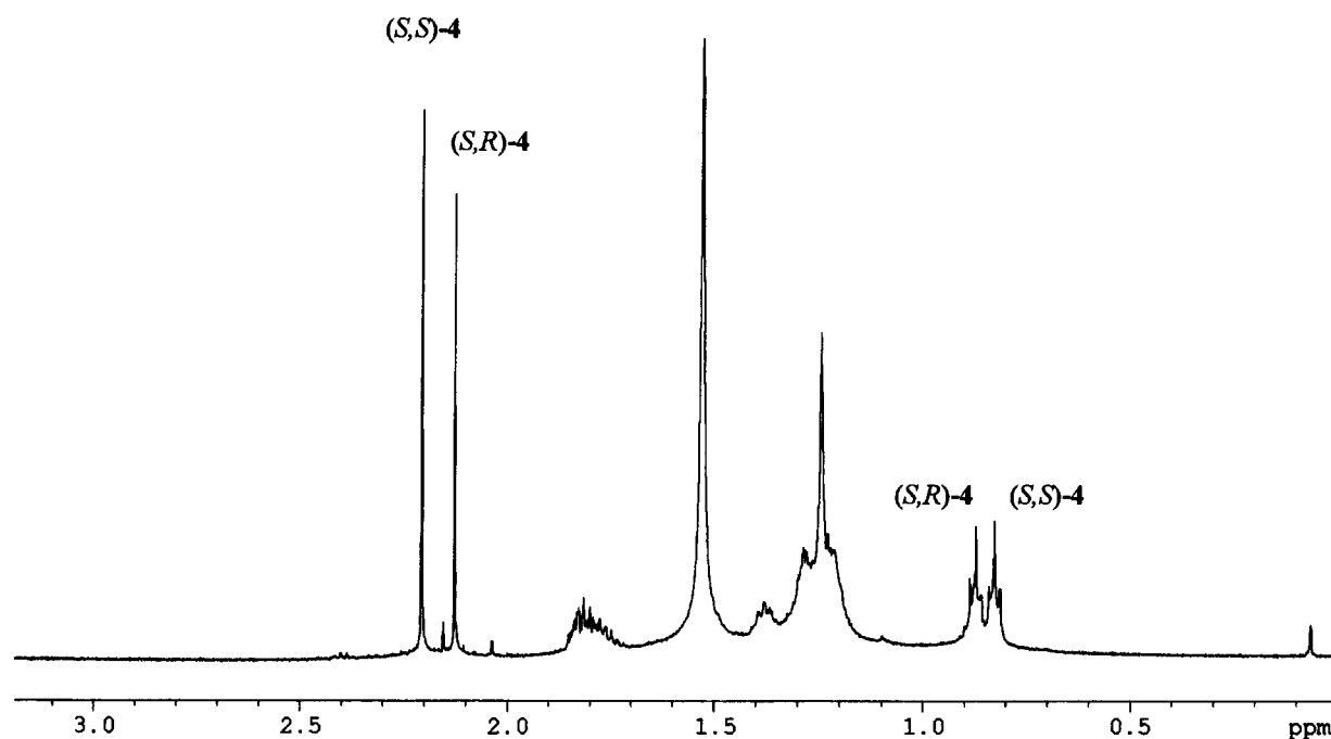
Figure 3. ^1\text{H} NMR spectrum (500 MHz, \text{CDCl}_3 ) of diastereomeric mixture of ( S )-MTPA esters of 3-hydroxy-2-hexanone ( 2 ).
