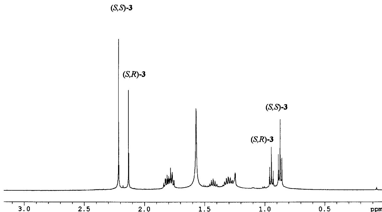
Figure 2. 1 H NMR spectrum (500 MHz, CDCl 3 ) of diastereomeric mixture of ( S )-MTPA esters of 3-hydroxy-2-hexanone ( 1 ).
